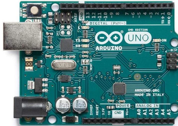
Figure 30: Arduino UNO R3
