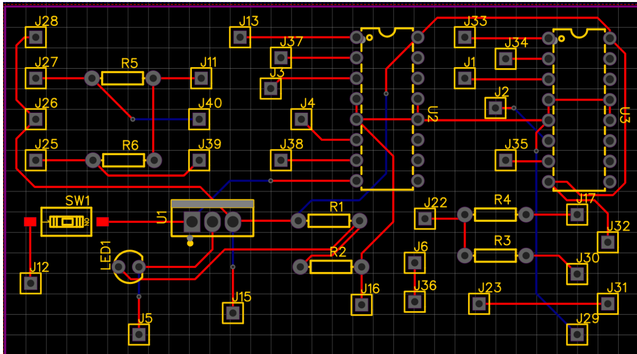
Figure 43: PCB
