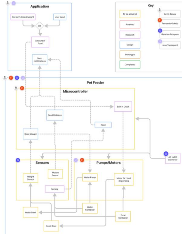
Figure 1: Block diagram of hardware and software
