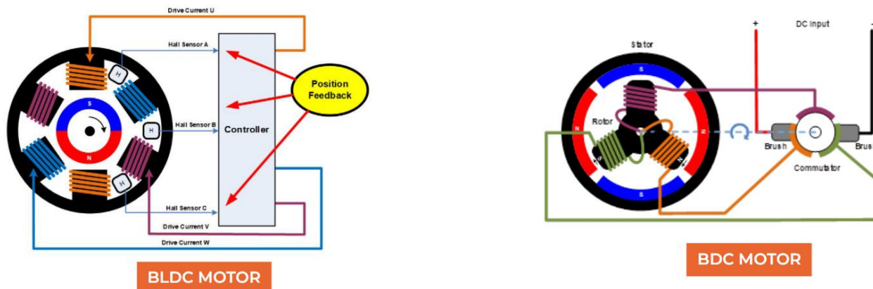
Figure 14: Difference between BLDC and BDC motors
